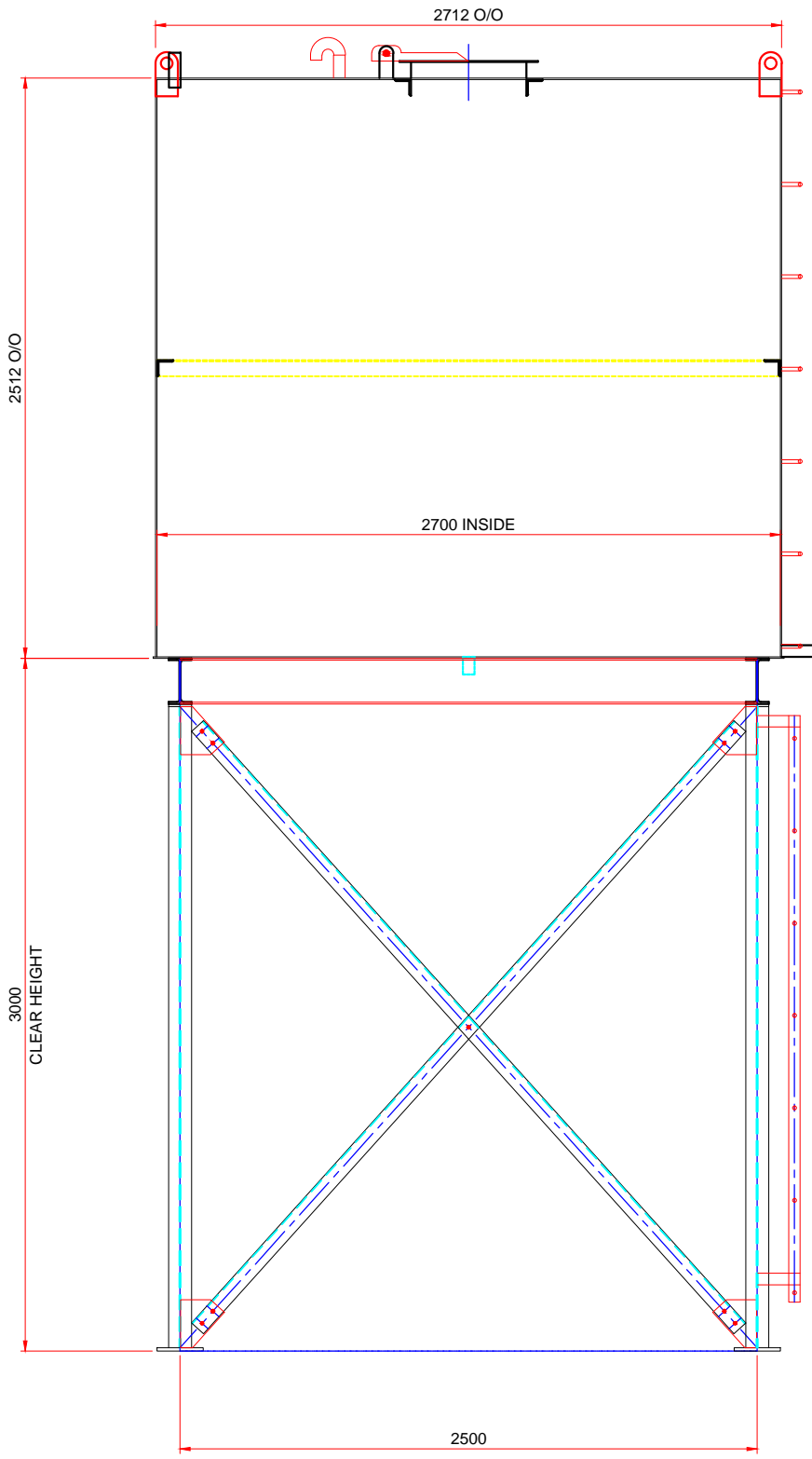
ELEVATION VIEW
